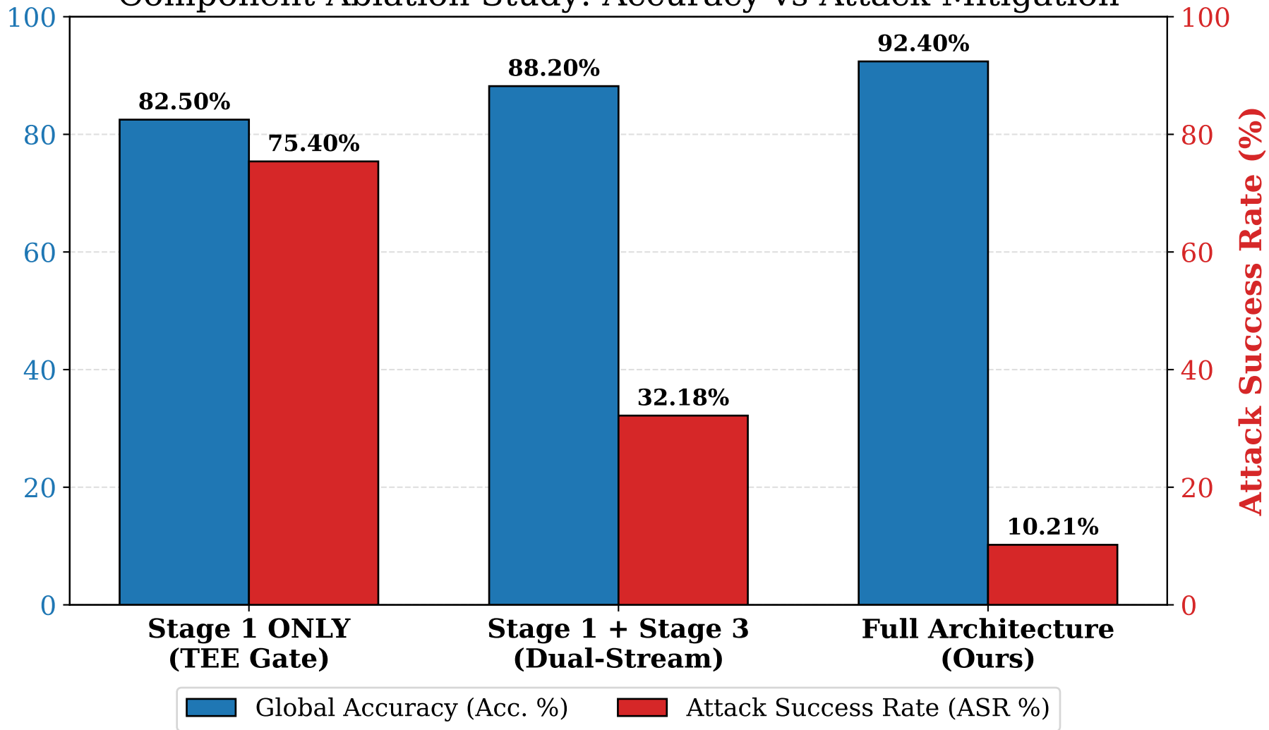
Component Ablation Study: Accuracy vs Attack Mitigation
